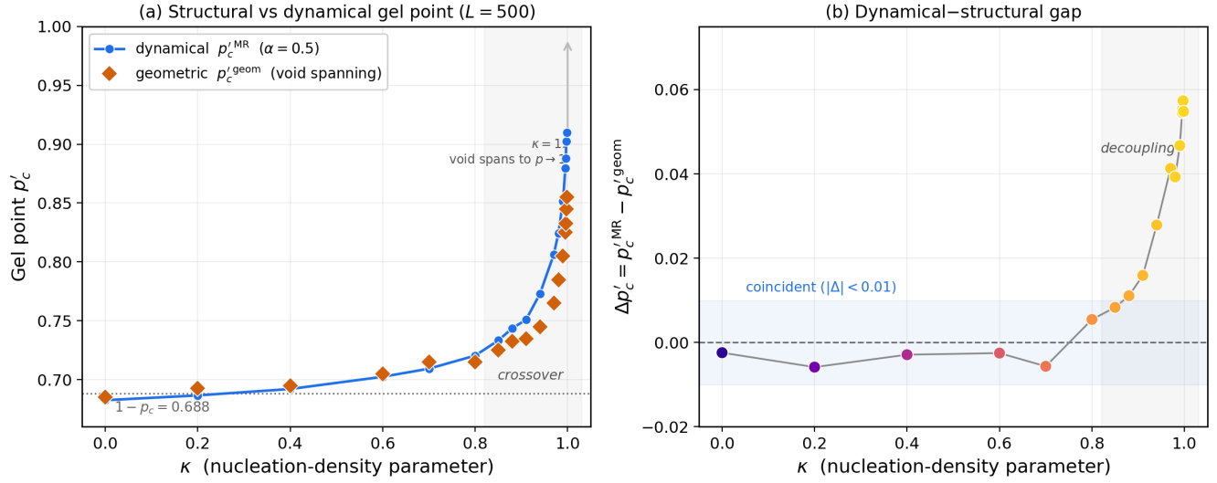
FIG. 4. The microrheological gel point is the void-percolation threshold. (a) Dynamical gel point p'_c{}^{\text{MR}} (the \alpha = 0.5 crossing) and the geometric void-spanning threshold p'_c{}^{\text{geom}} (loss of a face-to-face spanning empty cluster), both at L = 500 . (b) Their difference \Delta p'_c = p'_c{}^{\text{MR}} - p'_c{}^{\text{geom}} : the two coincide to within the p -grid resolution for \kappa \lesssim 0.8 and decouple through the Eden crossover, the dynamical point lagging the structural one. At \kappa = 1 the void of a single compact cluster spans until p \rightarrow 1 (no finite- p threshold).
